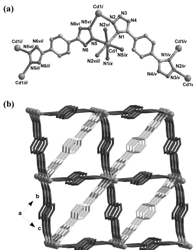
Figure 1. a) X-ray crystal structure of 1 showing the coordination environment of the Cd II ion and the coordination modes of BDT 2- ions. (Symmetry codes: i = −0.5 + x , 1.75 − y , 0.25 − z ; ii = −0.5 + x , −0.5 + y , z ; iii = x , 1.25 − y , 0.25 − z ; iv = 1 − x , 2 − y , − z ; v = 1.5 − x , 0.25 + y , −0.25 + z ; vi = 0.25 − x , y , 0.25 − z ; vii = 0.25 − x , 1.25 − y , z ; viii = 0.5 + x , 1.75 − y , 0.25 − z ; ix = 0.75 − x , 1.75 − y , z ). b) Packing diagram showing the 3D crystal structure of 1 . Lattice H 2 O molecules have been omitted for clarity.
