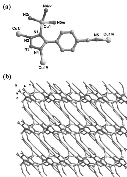
Figure 4. X-ray crystal structure of 4 showing the coordination environment of the Cu I ion and the coordination modes of the BNT - ions. (Symmetry codes: i = 1 - x, -y, -z ; ii = 1 - x, -0.5 + y, 0.5 - z ; iii = 2 - x, 2 - y, 1 - z ; iv = 1 - x, 0.5 + y, 0.5 - z ). b) The 3D structure of 4 .
